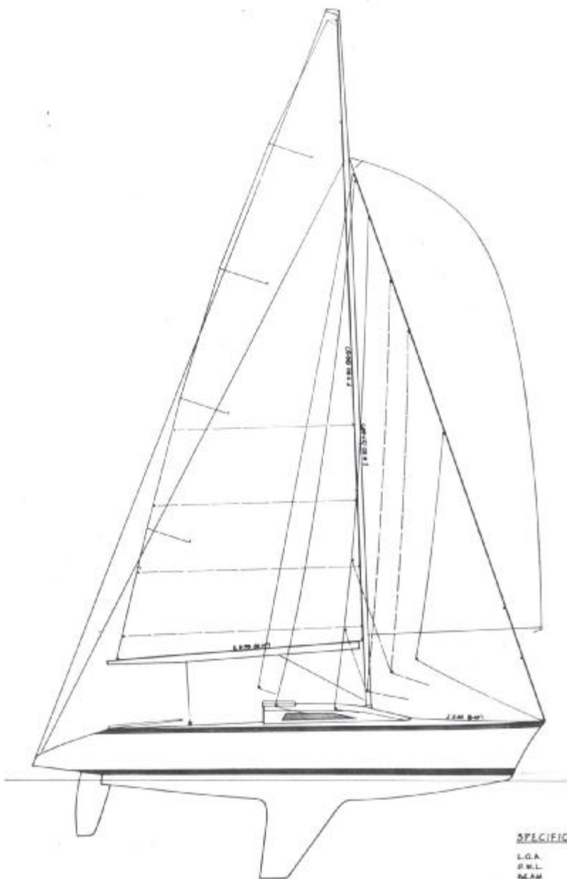
SAIL PLAN
