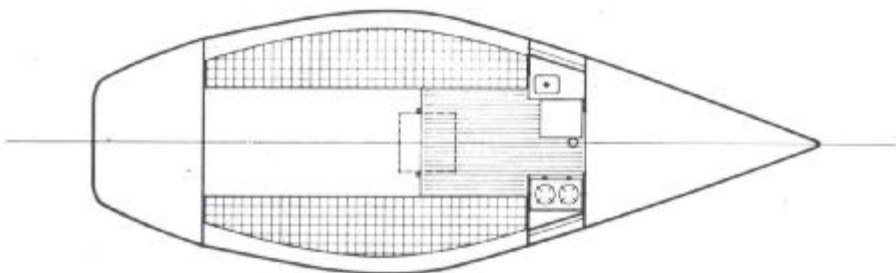
ARRANGEMENT
