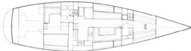
ARRANGEMENT
