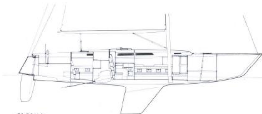
PROFILE
