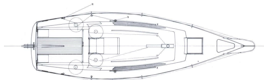
DECK LAYOUT.
