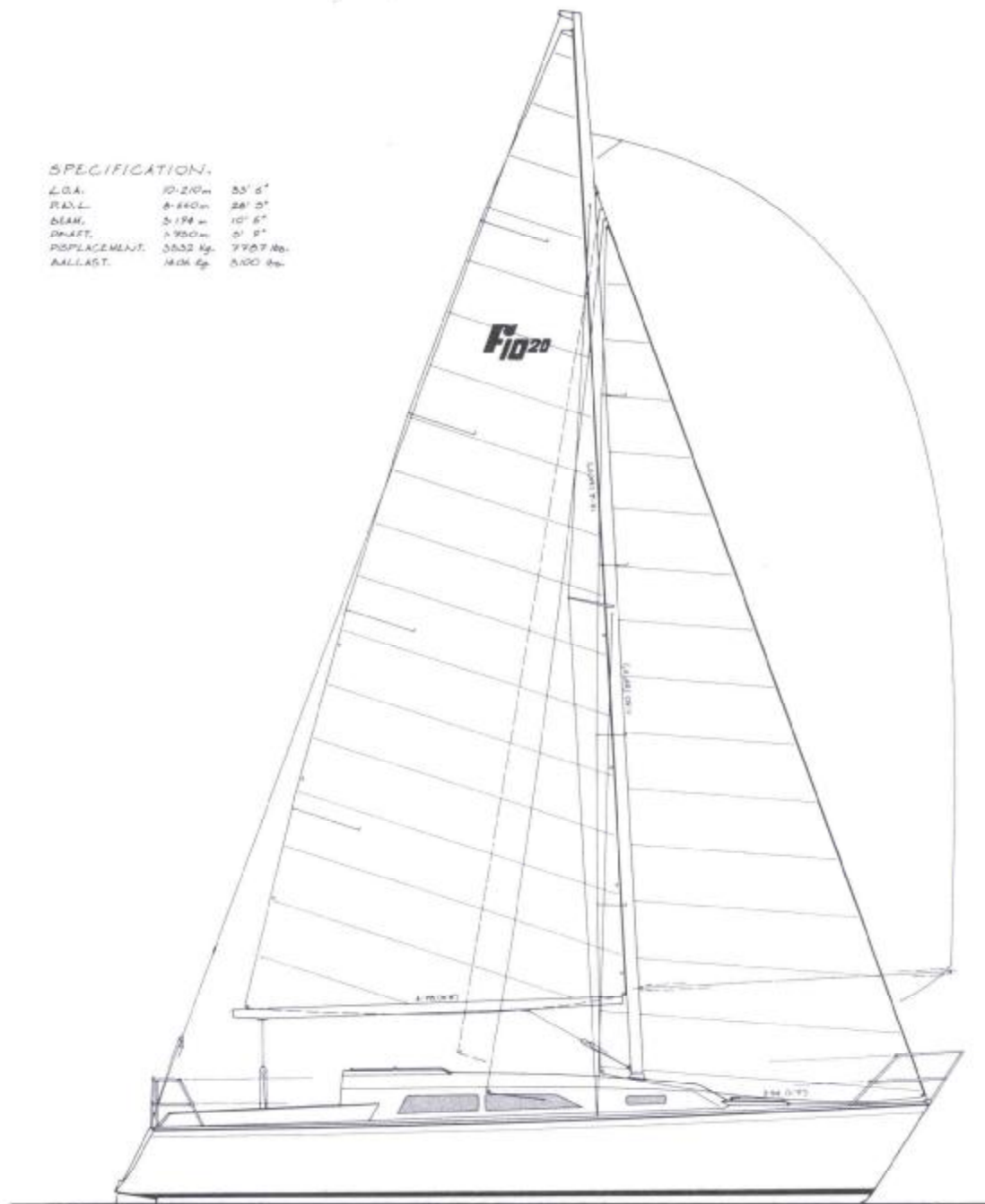
PROFILE.
