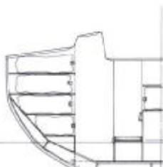
SECTION BY STATION #1.1
