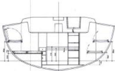
SECTION BY STATION #1.0
