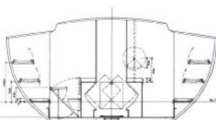
SECTION BY FRAME 10
