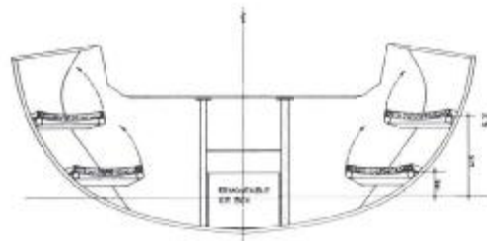
SECTION AT STN. 6.04
