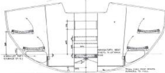
SECTION AT STN 7
