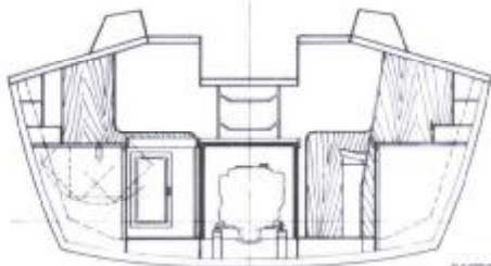
SECTION AT FRAME 3.
