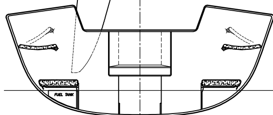
SECTION AT STN 7
