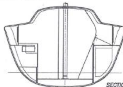
SECTION AT STN 4 1/2
