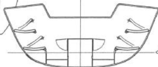
SECTION at Stn 7
