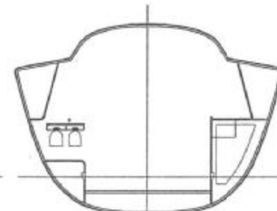
SECTION at Stn 4
