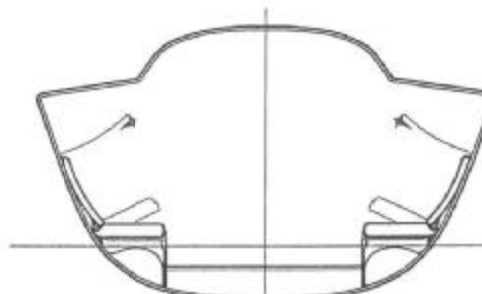
SECTION at Stn 5
