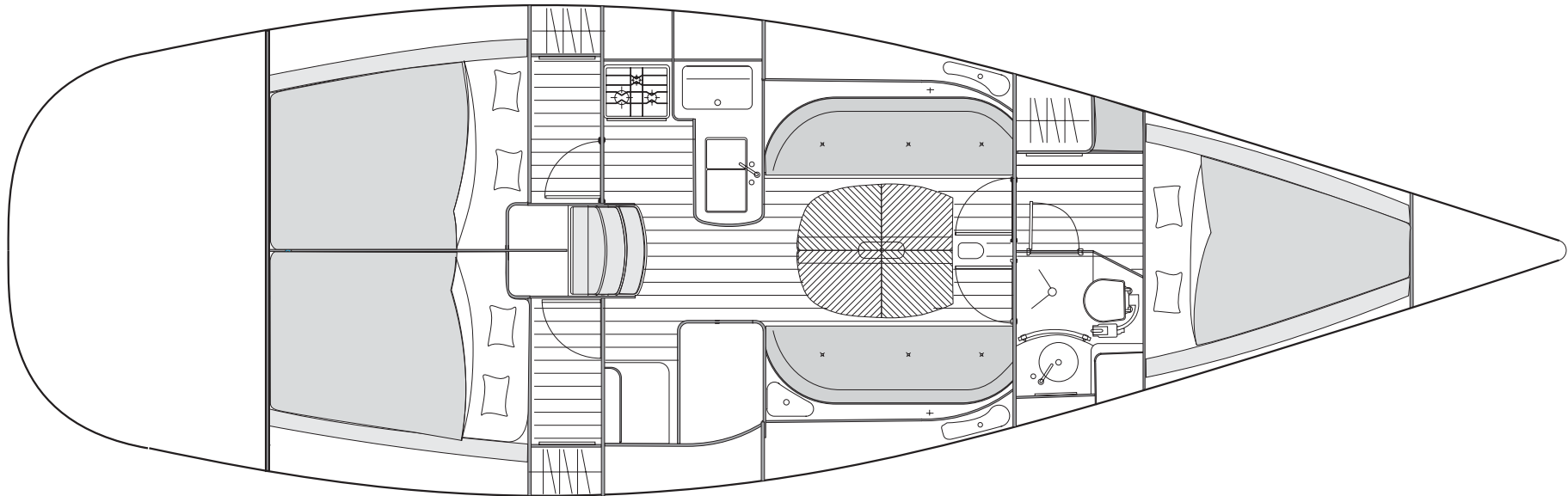
FIRST 40.7 AMENAGEMENT 3 cabines / 3 cabins layout
