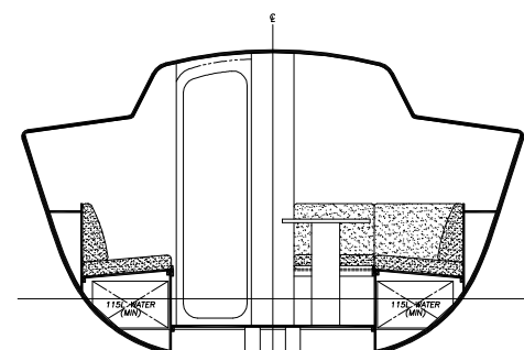
SECTION AT 5.
