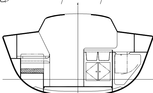
SECTION AT 6.5.
