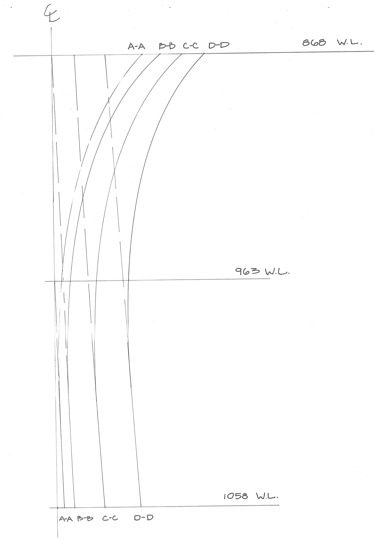
FILLET SECTIONS
