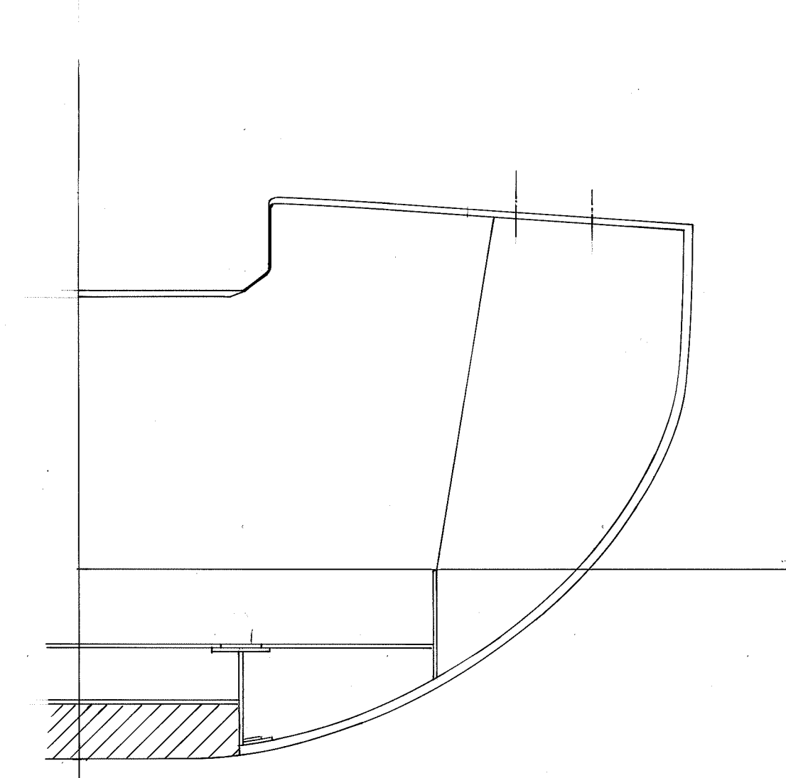
BULKHEAD 250 FWD. OF STN 6
