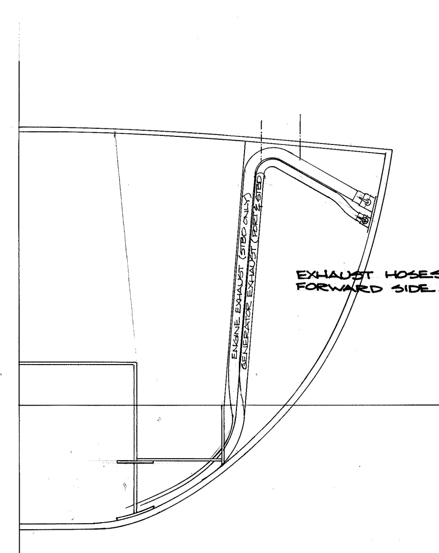
BULKHEAD 140 FWD. OF STN 4
